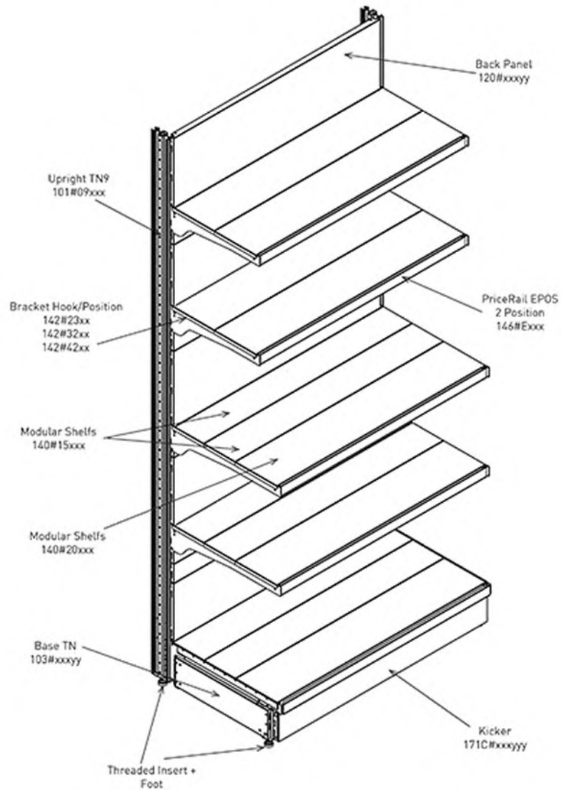
R-Series Wall Shelving
