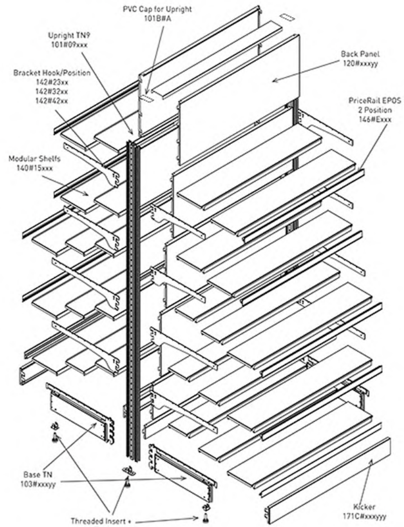
R-Series Gondola (Exploded View)
