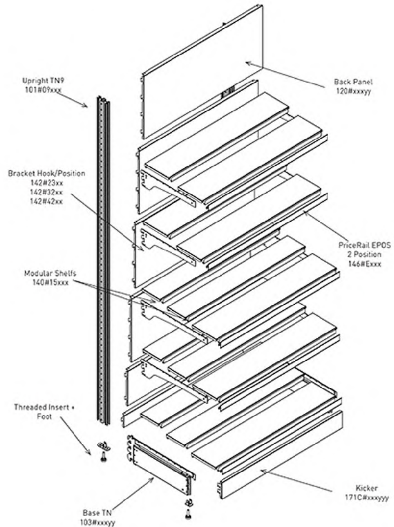
R-Series Wall Shelving (Exploded View)
